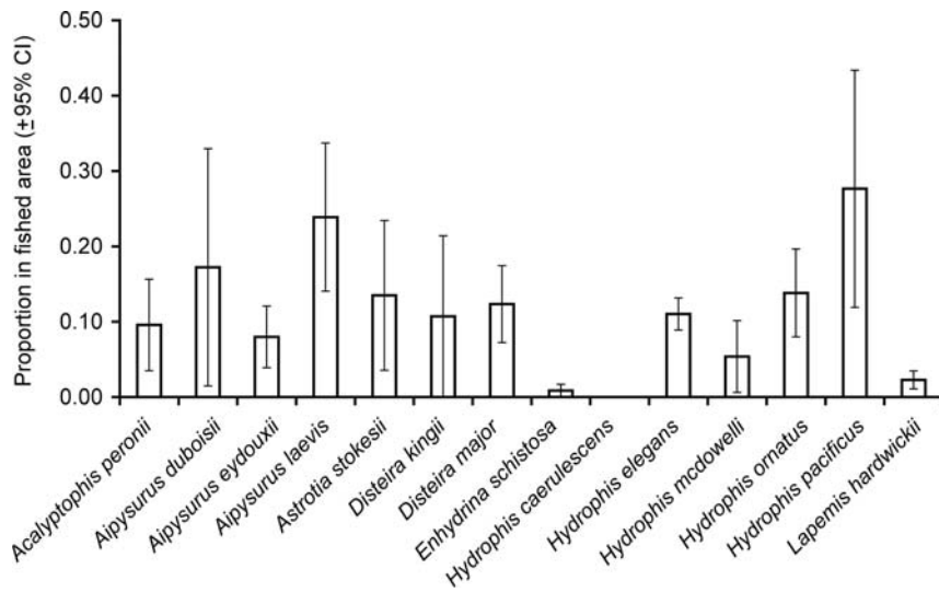
Figure 2. The estimated proportion of sea snake abundances in the commercially fished area ( \pm 95\% CI). Hydrophis caerulescens was only caught in commercially unfished areas.
