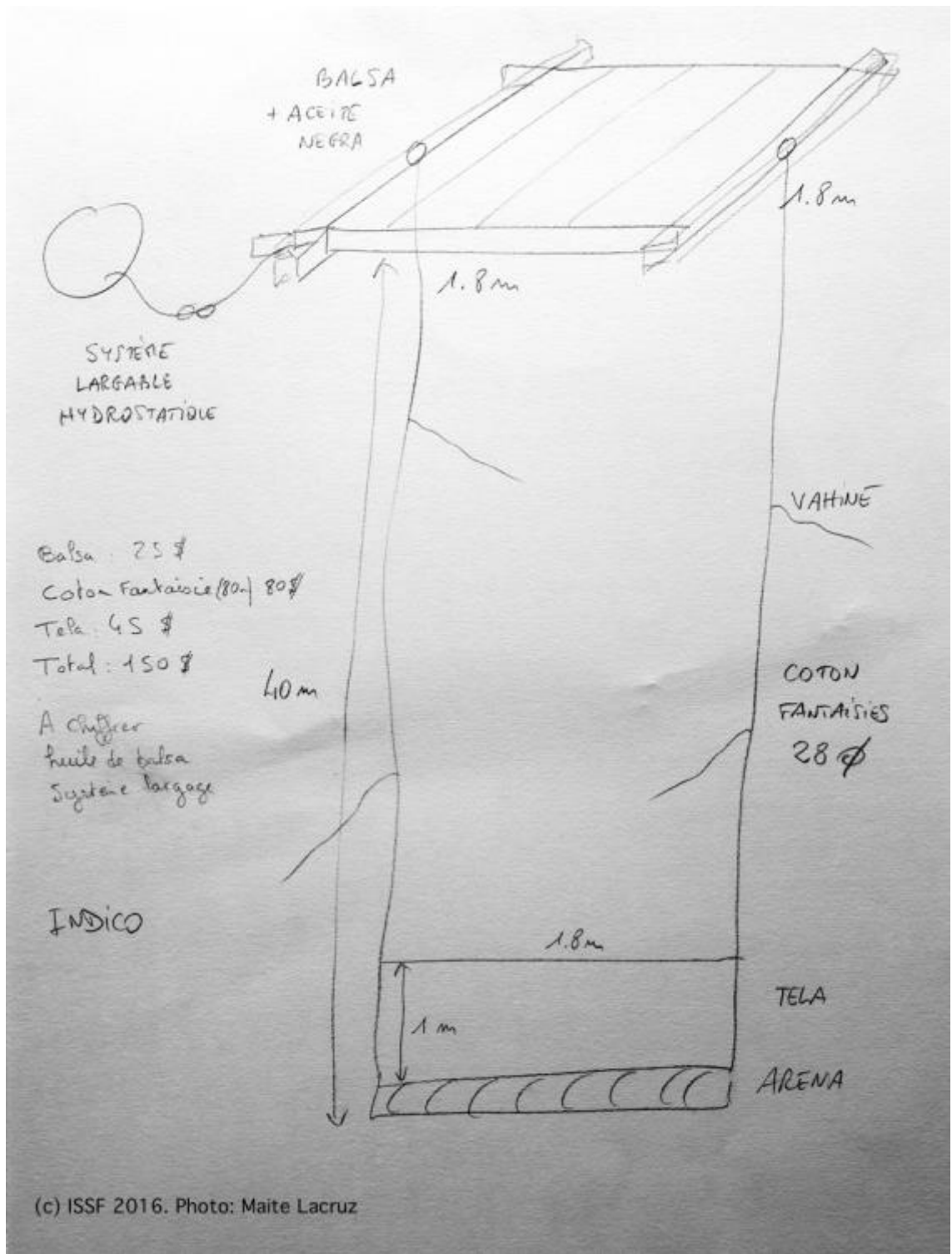
Fig. 10. Biodegradable FAD designed during the workshop for the Indian Ocean.
