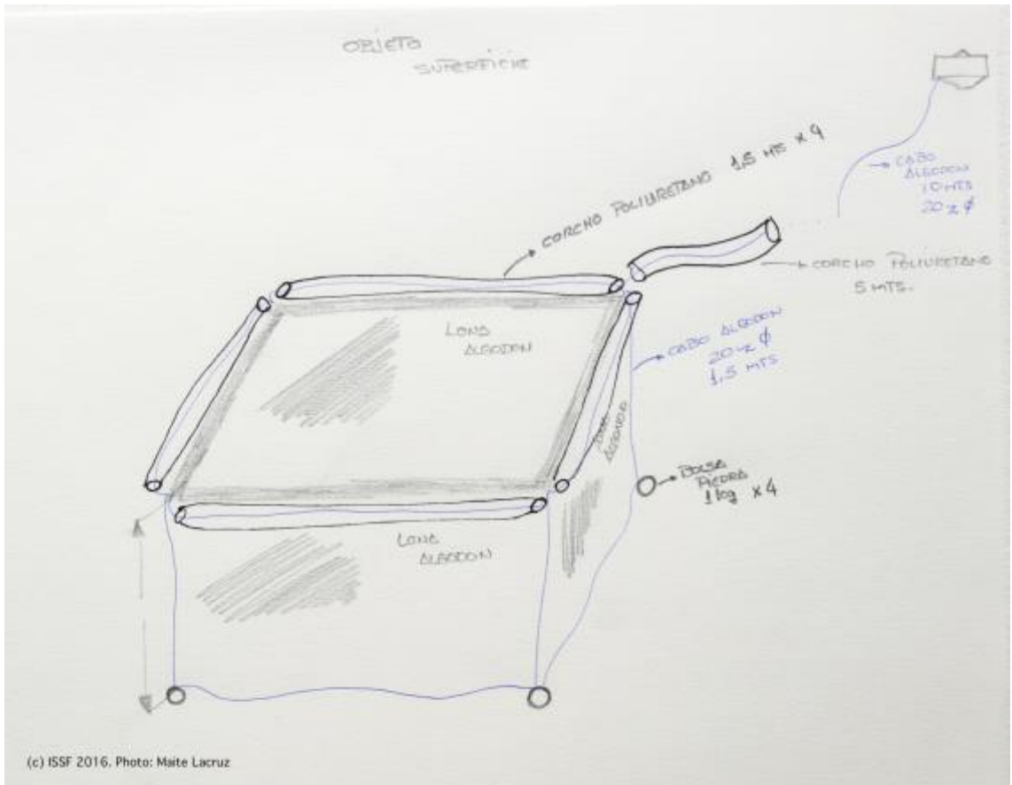
Fig. 12. Biodegradable FAD designed during the workshop for the Indian Ocean (shallow structure).
