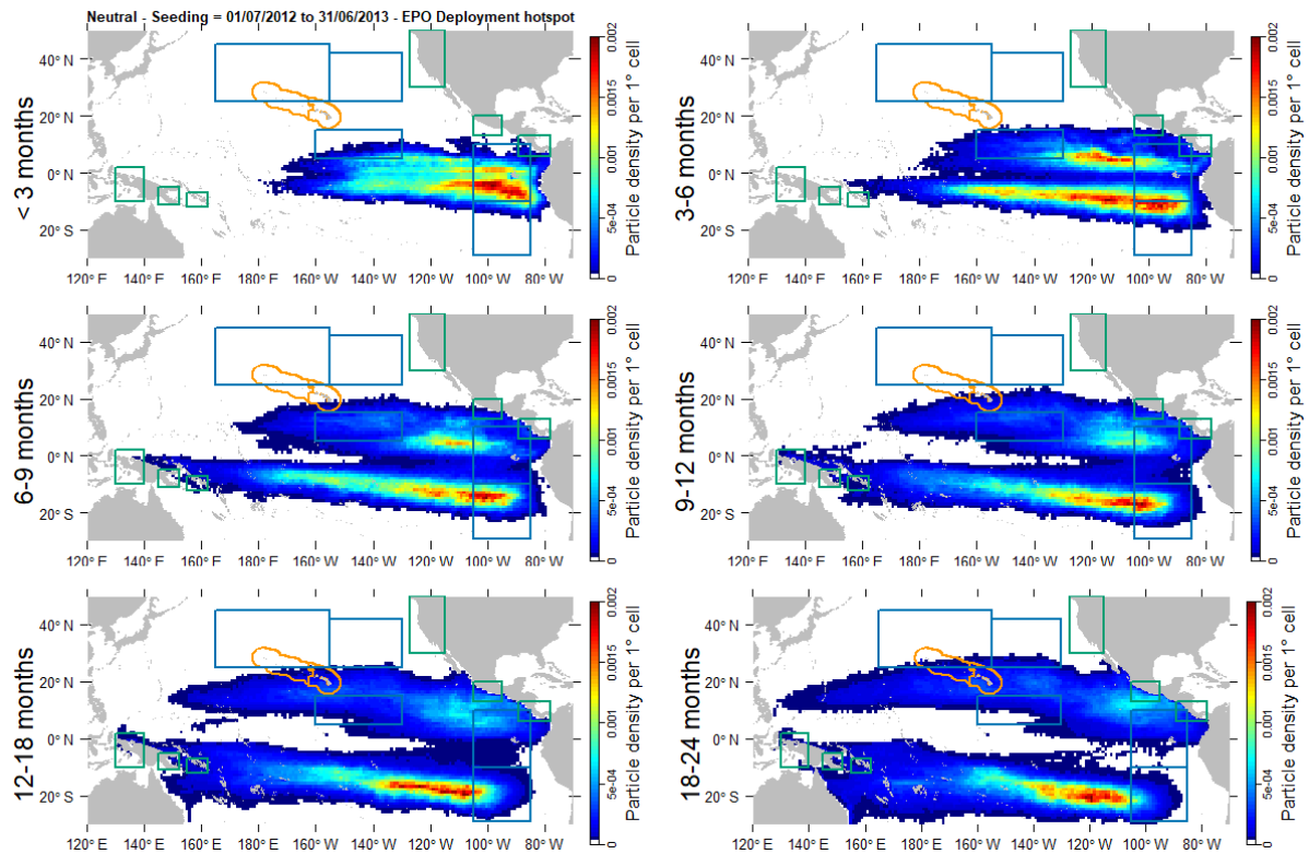
Figure 6. Spatial probability density for virtual particles deployed in the EPO FAD deployment hotspots during a Neutral period (01/07/2012 to 31/06/2013) during six drifting time bins after deployment.
