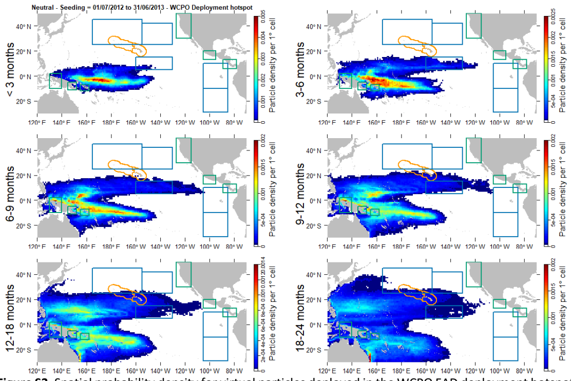
Figure S3. Spatial probability density for virtual particles deployed in the WCPO FAD deployment hotspots during a Neutral period (01/07/2012 to 31/06/2013) during six drifting time bins after deployment.
