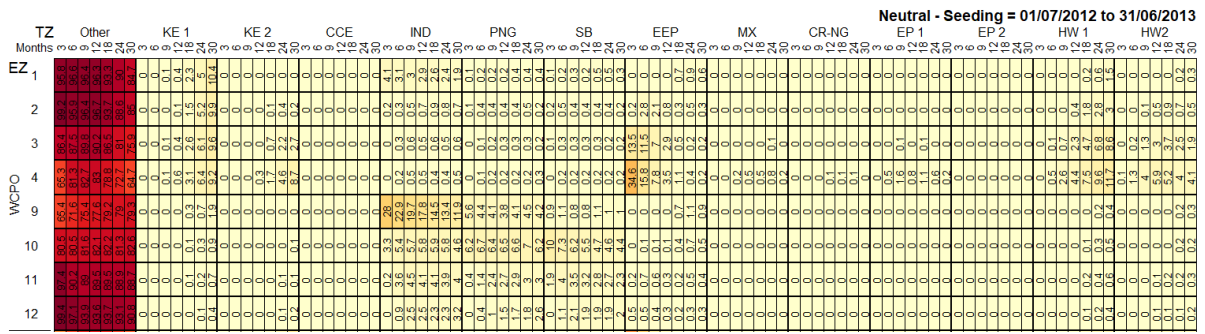
Figure S1. Percentage connectivity matrix of virtual particles in the time-forward simulation during an ENSO Neutral period (01/07/2012 to 31/06/2013) by Turtle Zones (TZ) against seeding in WCPO Equatorial Zones (EZ) and separated by drift time in months. Cells are coloured by proportion of simulated particles arriving in each TZ by drift-time.
