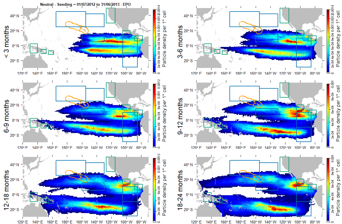
Figure 4. Spatial probability density for virtual particles deployed in the whole equatorial region in the EPO (EZs 5–8 and 13–16) during a Neutral period (01/07/2012 to 31/06/2013) during six drifting time bins after deployment.
