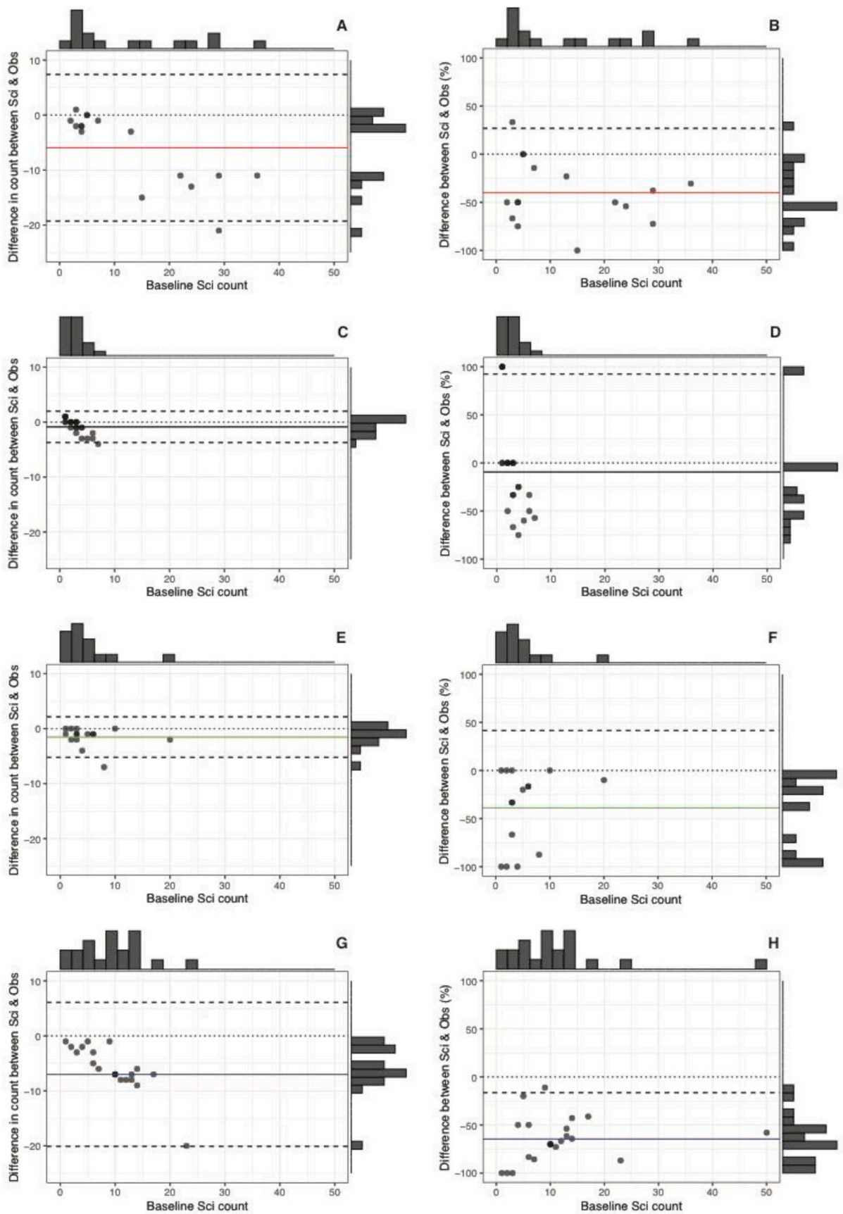
Fig. 1. Bland and Altman plots illustrating the difference in shark counts by scientists (Sci) and observers (Obs) in numbers of sharks on the left (A,C,E,G) and by percentages on the right (B,D,F,H) per set for WCPO1, WCPO2, AO and IO EMS cruises. Solid lines represent the mean bias, dotted lines represent the limits of agreement ( 2 \times SE ). The marginal histograms denote the frequency distributions of the X and Y variables.
