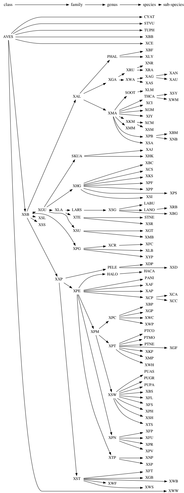
Figure A-3: Hierarchy of codes used to define the species or species groups during the bird counts. This hierarchy was used when processing the data to resolve discrepancies when two or more codes were used by the observers to define a species or species group. (See Table 1 for the species and species groups defined by each code.)
