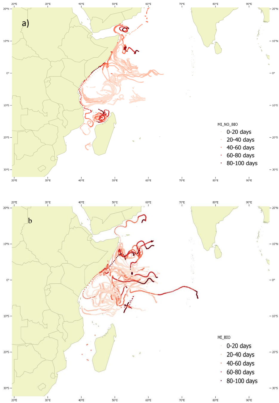
Figure 5. Trajectories followed by a) non-biodegradable FADs and b) biodegradable FADs.
