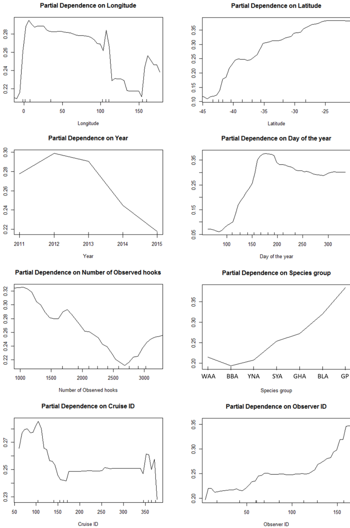
Figure 4. Albatross mitigation model. Figures show that the partial dependences associated with changes of each variation. The Y axis indicates the partial dependence. The larger value means lower probabilities of bycatch.
