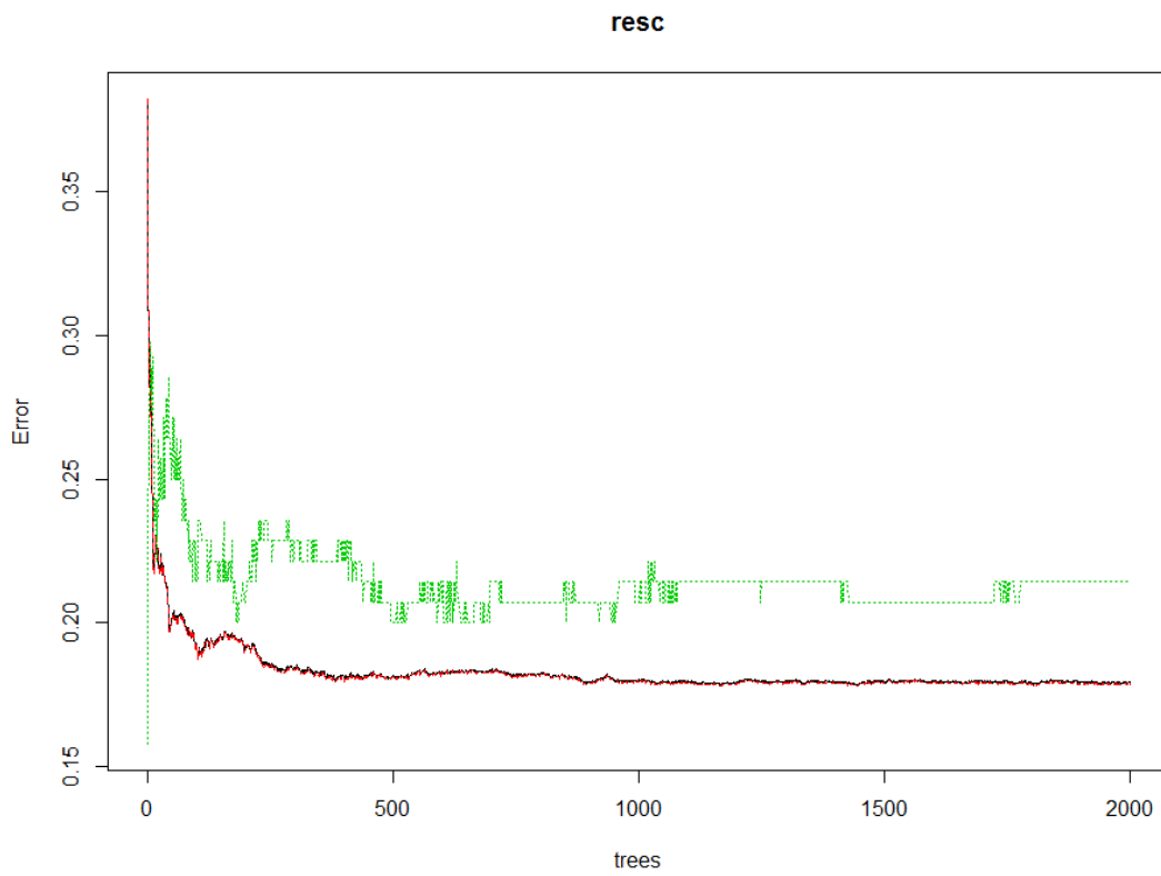
Figure 1d. Petrel mitigation measure model
