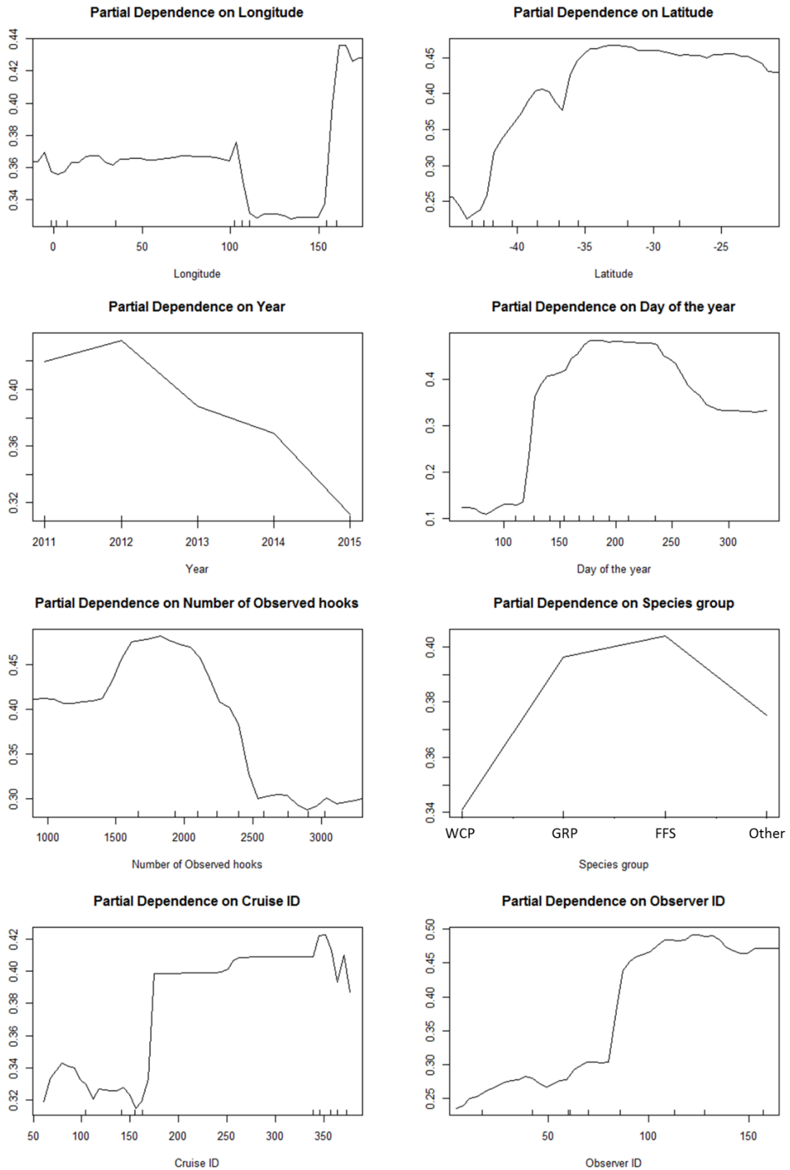
Figure 6. Petrel mitigation model. Figures show that the partial dependences associated with changes of each variation. The Y axis indicates the partial dependence. The larger value means lower probabilities of bycatch.
