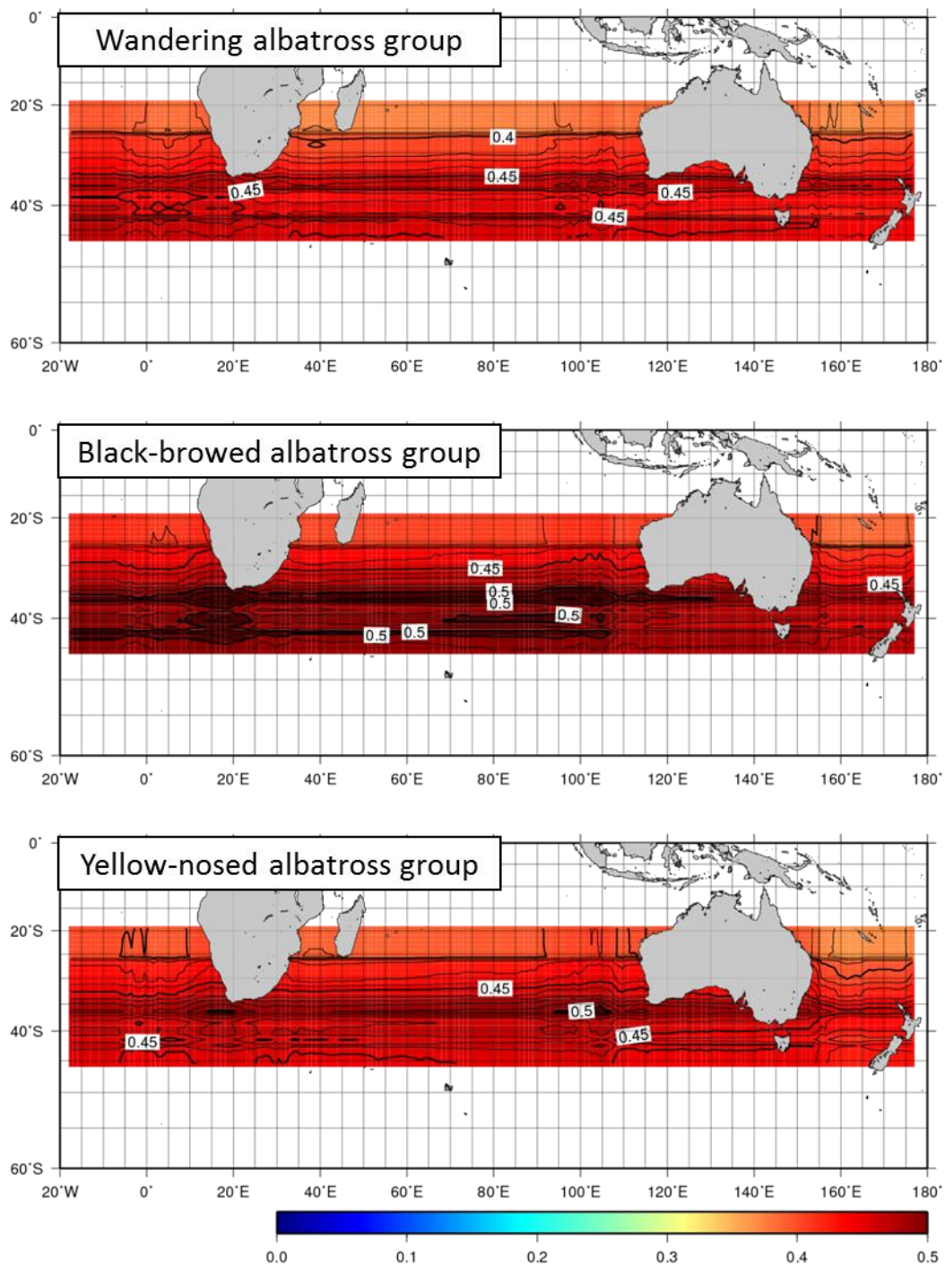
Appendix 1, Figure 7. Distribution of bycatch occurrence rate predicted by albatross model or petrel model. Color shows the degree of bycatch occurrence rate with indicating that red is high rate.
