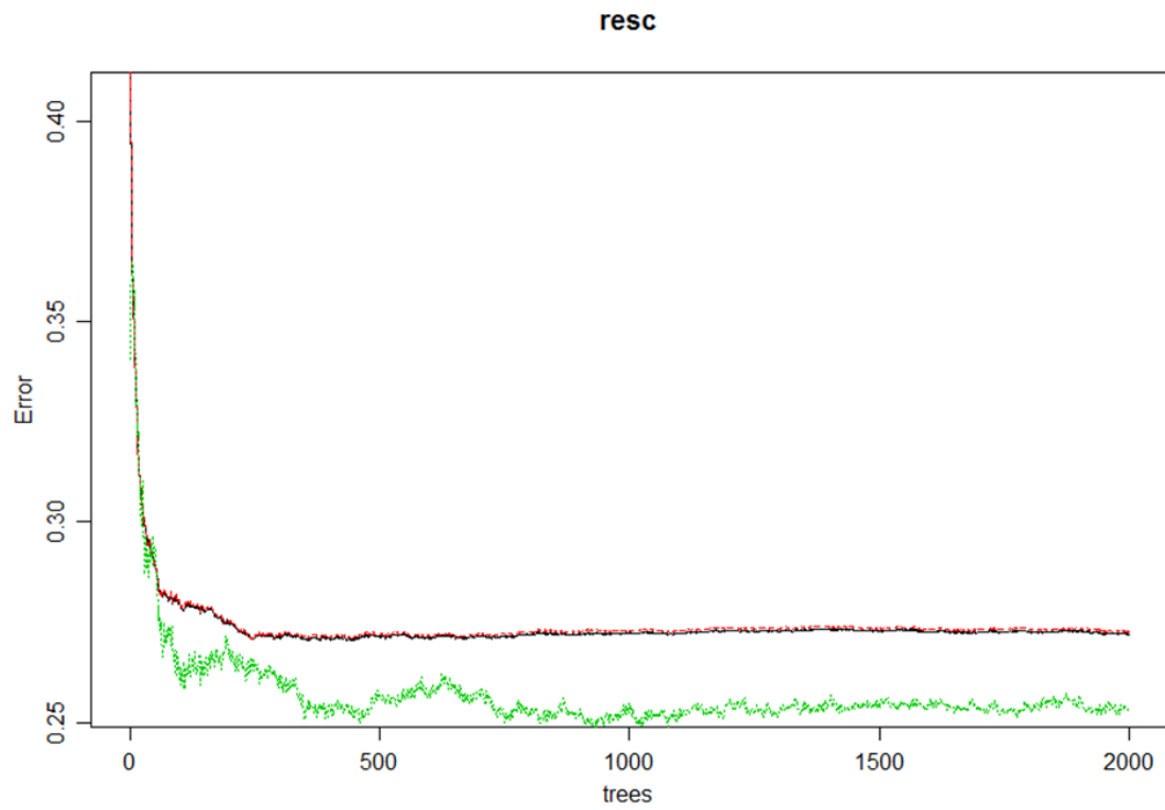
Figure 1a. Albatross model.
