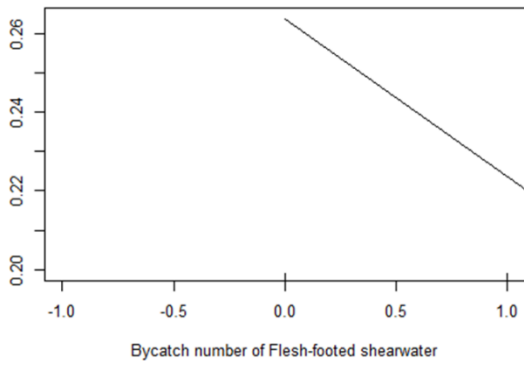
Partial Dependence on Use of Weighted blanch line
