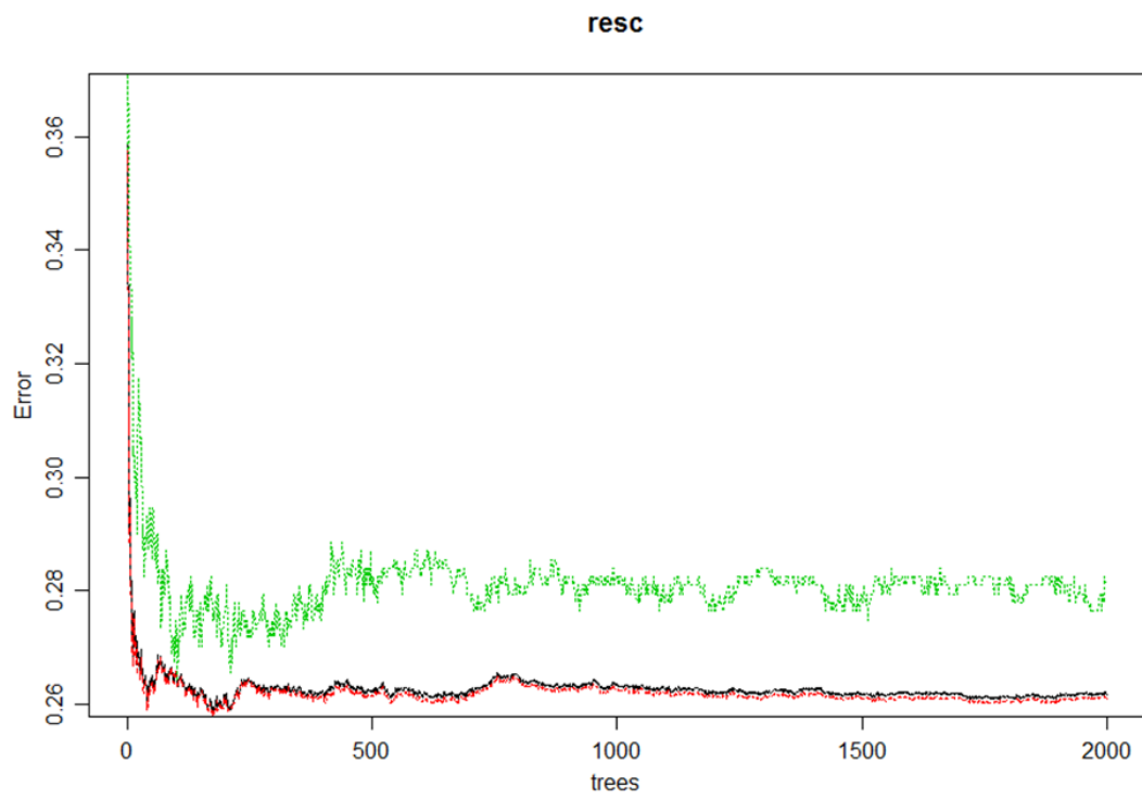
Figure 1b. Albatross mitigation measure model.
