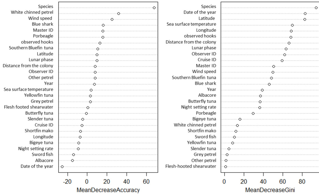
Figure 2a. Albatross model.
