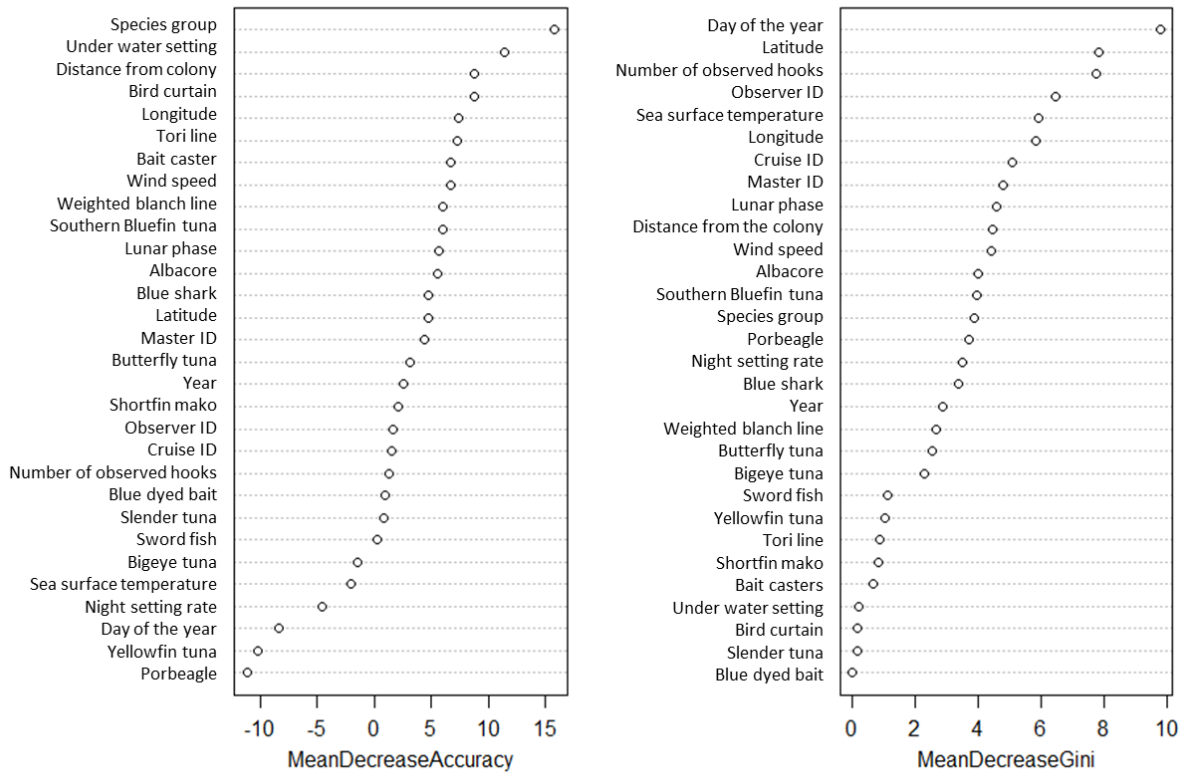
Figure 2d. Petrel mitigation model.
