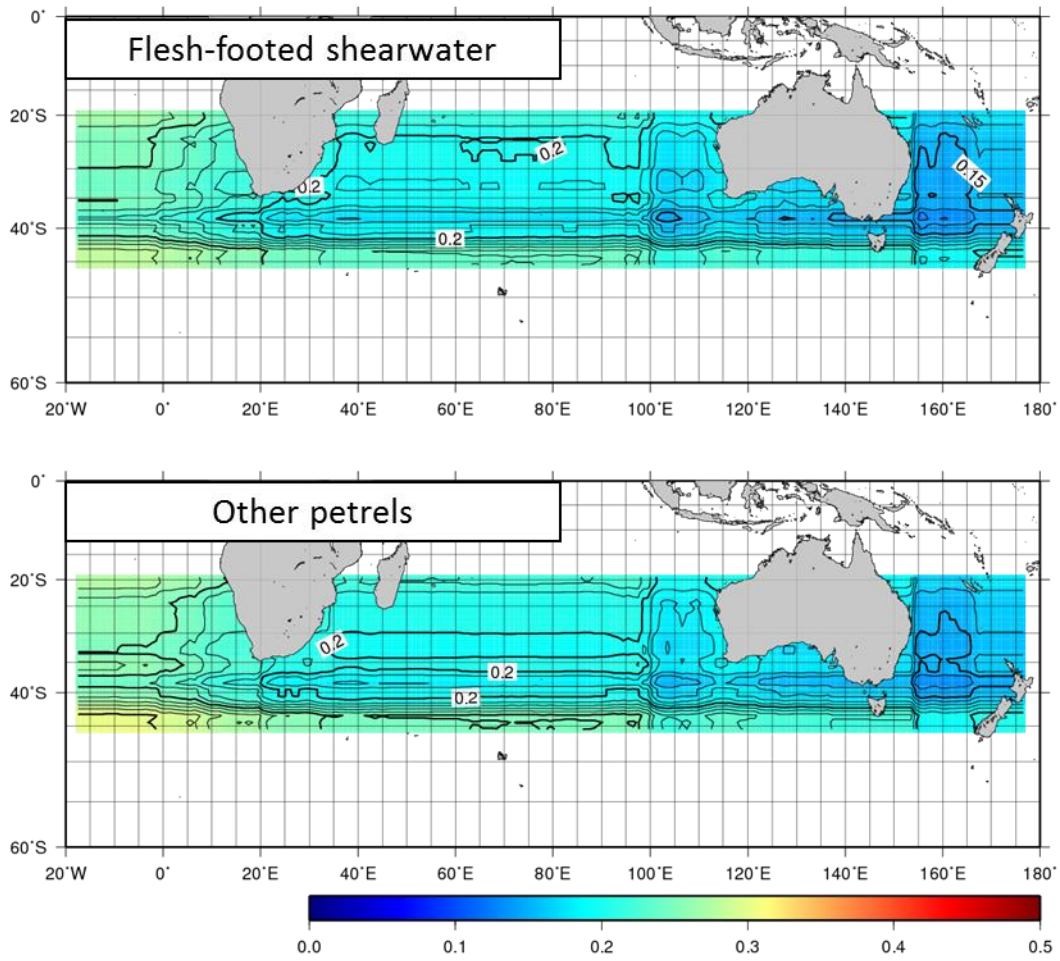
Appendix 1, Figure 7. Continued.
