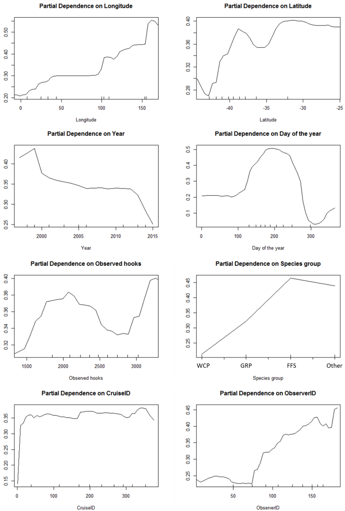
Figure 5. Petrel model. Figures show that the partial dependences associated with changes of each variation. The Y axis indicates the partial dependence. The larger value means lower probabilities of bycatch.
