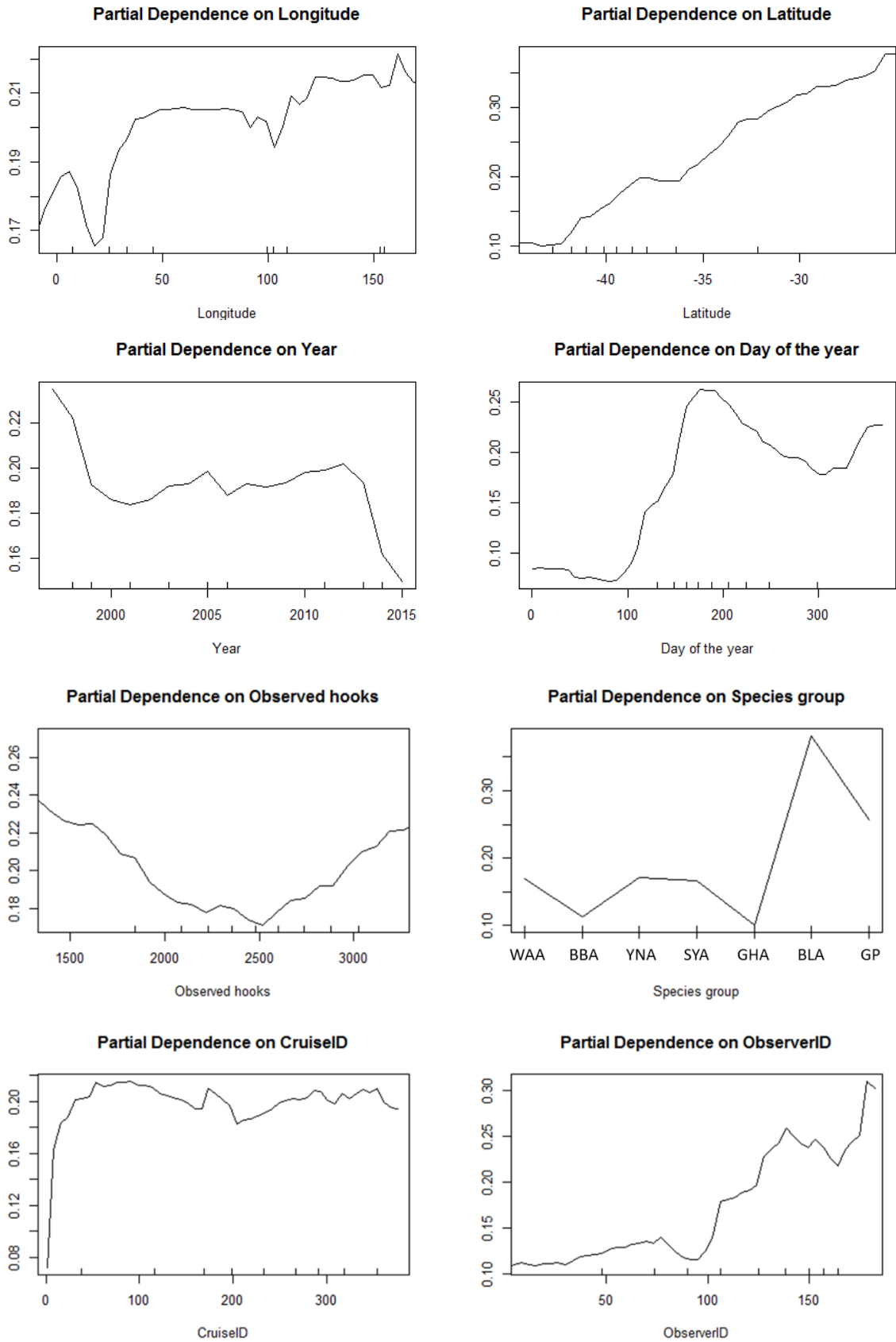
Figure 3. Albatross model. Figures show that the partial dependences associated with changes of each variation. The Y axis indicates the partial dependence. The larger value means lower probabilities of bycatch.
