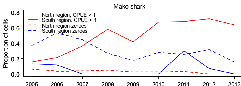
Figure 7: Mako shark distribution indicators. Proportions of 0.5 degree rectangles having CPUE greater than 1 per 1000 hooks, and proportions of rectangles having zero catches, for North and South regions by fishing year, based on estimated catches (processed and discarded combined) reported on TLCERs.
