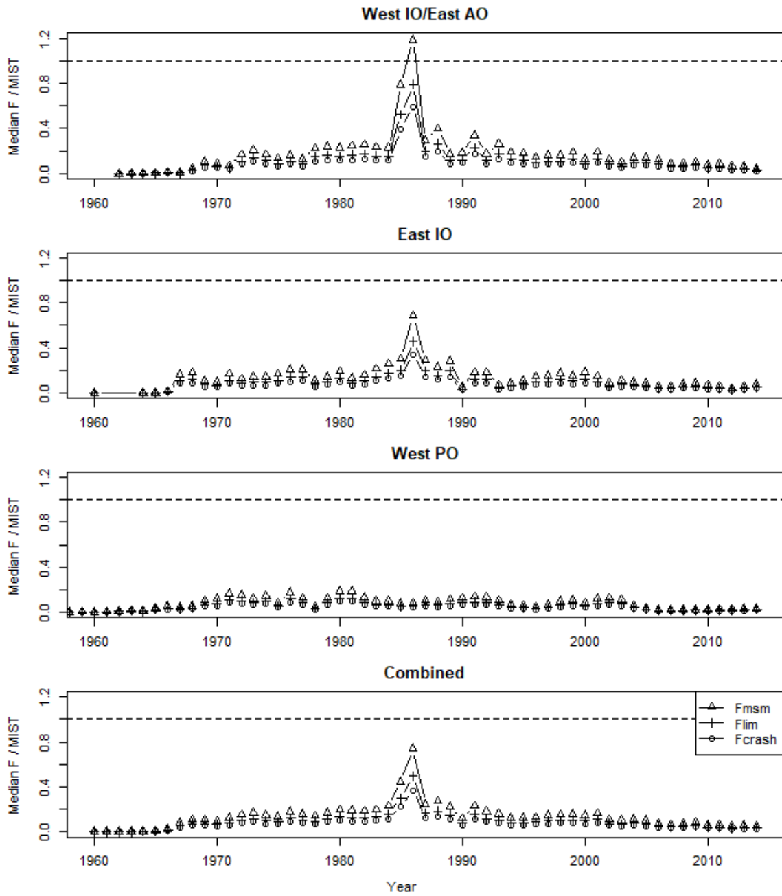
Figure ADD2: F-ratio plots showing the median values of F / MIST by year, for the three versions of the MIST ( F_{msm} , F_{lim} , and F_{crash} ) for each of the three regions and for the three regions combined (the assessment area). Note that the F-ratio is almost always below 1, indicated by the horizontal dotted line.
