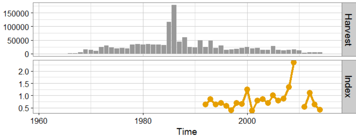
Figure 19. Catch and abundance data.
