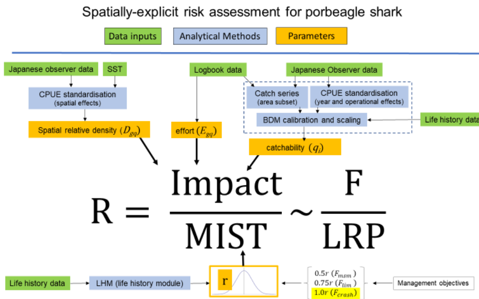
Figure 17. Conceptual representation of data inputs, analytical methods and key parameters used in spatially-explicit risk assessment of the Southern Hemisphere porbeagle shark. BDM = Bayesian state-space biomass dynamics model. The dashed outline box represents analytical methods applied to a region subset of the available data.
