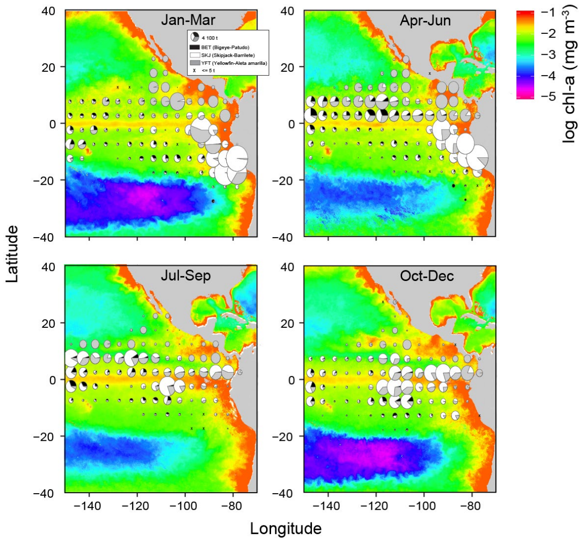
FIGURE J-11. Mean log chlorophyll-a concentration (in \text{mg m}^3 ) for each quarter during 2021 with catches of tropical tunas overlaid. Chlorophyll data obtained from NOAA CoastWatch on January 20, 2022, “Chlorophyll, NOAA, VIIRS, Science Quality, Global, Level 3, 2012-present, Monthly”, NOAA NMFS SWFSC ERD, https://coastwatch.pfeg.noaa.gov/erddap/info/nesdisVHNSQchlaMonthly/index.html .
