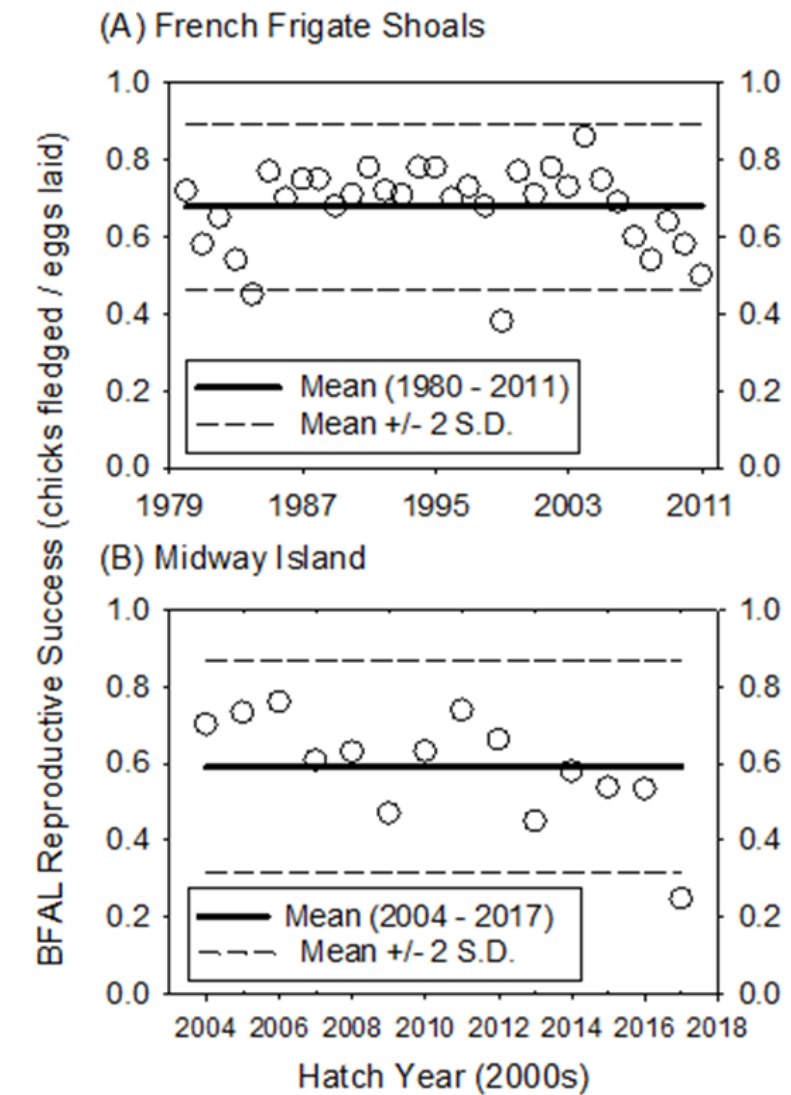
Figure 28. Time series of BFAL reproductive success at two study sites. To highlight interannual variability, yearly values are compared to the mean + 2 standard deviations.
