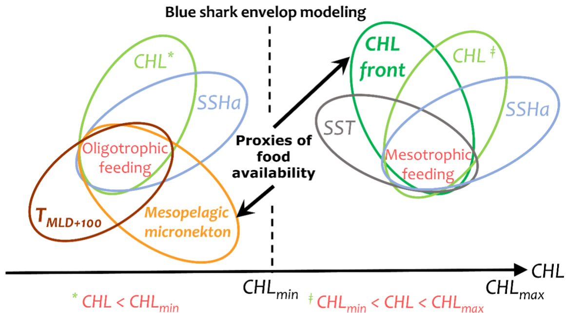
Figure 1. Scheme of the blue shark envelope modeling linking the environmental variables and the ecotrophic types of feeding in oligotrophic ( CHL < CHL_{min} ) and mesotrophic ( CHL_{min} < CHL < CHL_{max} ) environments with mesopelagic micronekton and productivity fronts (chlorophyll-a horizontal gradients) as feeding proxies, respectively. The abiotic variables (SST, T_{mld+100} and SSHa) were used to exclude unsuitable environments. CHL: surface chlorophyll-a content; SST: sea surface temperature; T_{mld+100} : Temperature 100 m below the mixed layer depth; SSHa: sea surface height anomaly.
