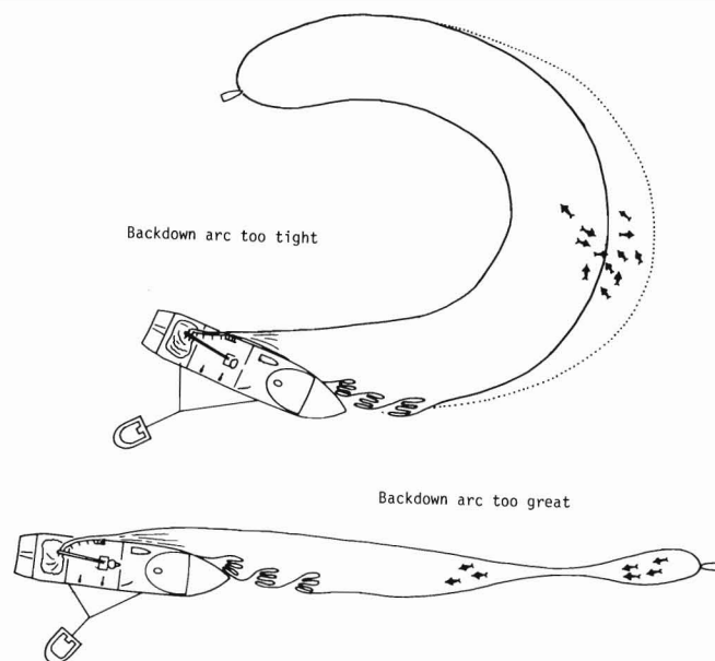
Figure 20. —Proper backdown arc insures efficient waterflow to maintain a wide and deep channel. Maintain correct radius of turn by changing the pulling position of the net skiff, rudder angle, and direction of bow thruster as necessary.
