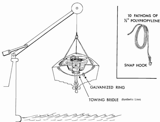
Figure 5.—Rigging for speedboat towing bridle. Note that the galvanized ring is free to slide the entire length of the towing bridle.
