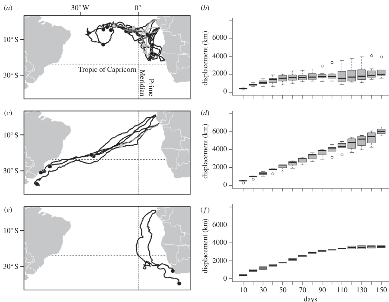
Figure 2. Movements and displacement time series of female leatherback turtles highlighting differing dispersal strategies. (a,c,e) Satellite-tracked movements and (b,d,f) box and whisker plots; boxes show 25th, 50th (median) and 75th percentiles (whiskers extend to the 2.5th and 97.5th percentiles, extremes are identified by empty circles), summarizing leatherback turtle displacement at 10-day intervals for up to 150 days from Gabon to South Atlantic habitats for the three dispersal groups: (a,b) habitats of the equatorial Atlantic; (c,d) habitats off South America, and (e,f) habitats off South Africa. (a) n = 15 ; (c) n = 6 ; (e) n = 2 .
