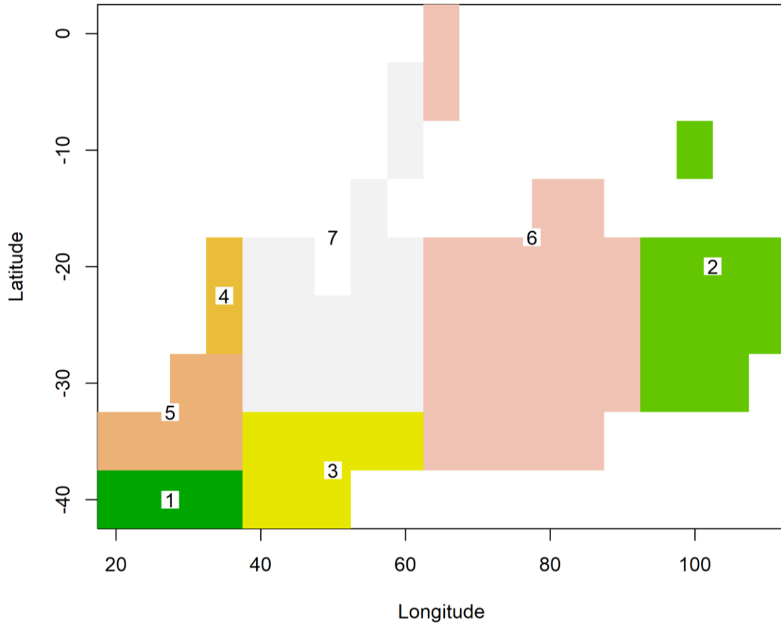
Figure 7. Spatial area stratification for the SMA CPUE captured by the Portuguese longline fleet in the Indian Ocean.
