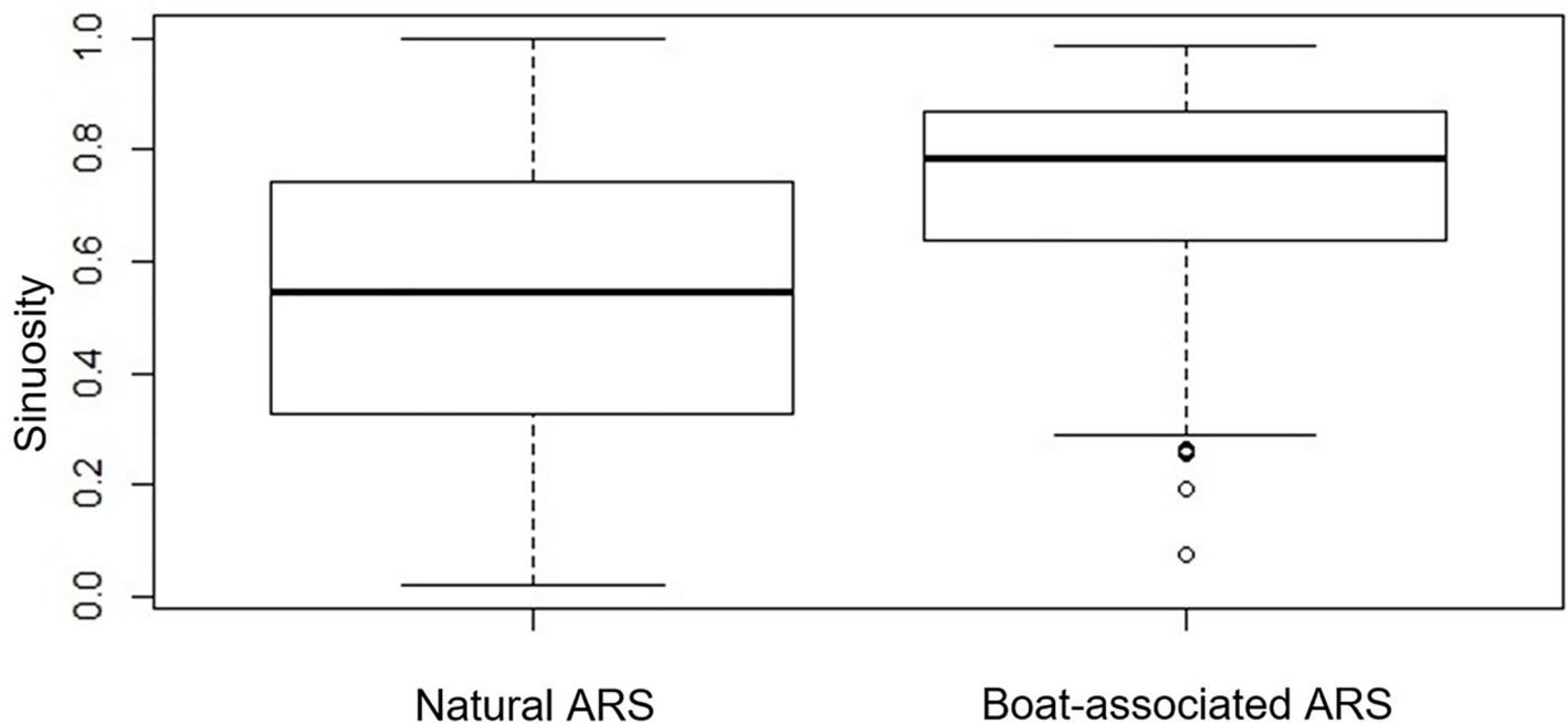
Fig 4. Sinuosity boxplot of small scales ARS: Natural ARS are significantly different than ARS associated with a boat.
