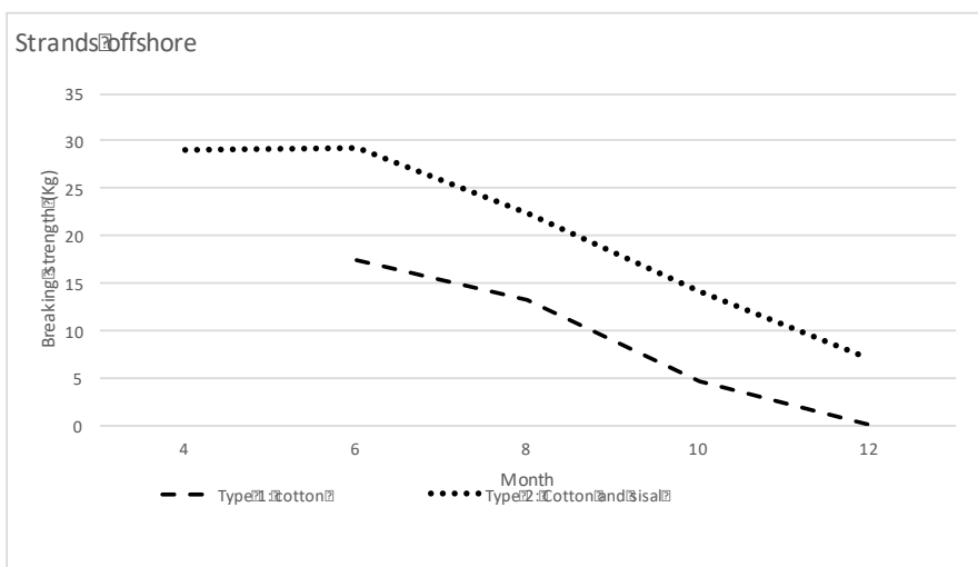
Figure 4. Biodegradable ropes' strands degradation with time. For those anchored in offshore waters (bottom) and within the lagoon (top).
