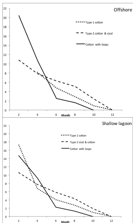
Figure 3. Biodegradable ropes' strings degradation with time. For those anchored in offshore waters (top) and within the lagoon (bottom).
