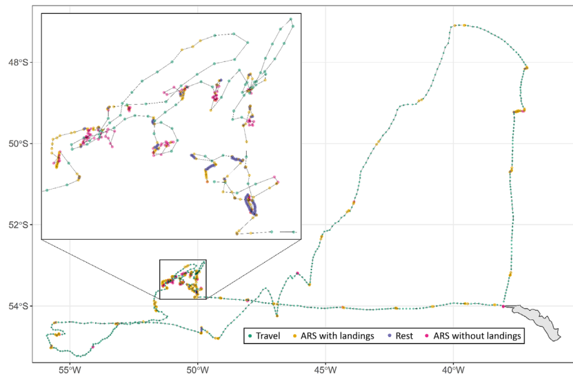
Figure 2 Example of one foraging trip of a wandering albatross tracked from Bird Island, South Georgia, during incubation in 2020, with regularised GPS locations coloured by behaviours derived from the 4-state hidden Markov model (HMM).
