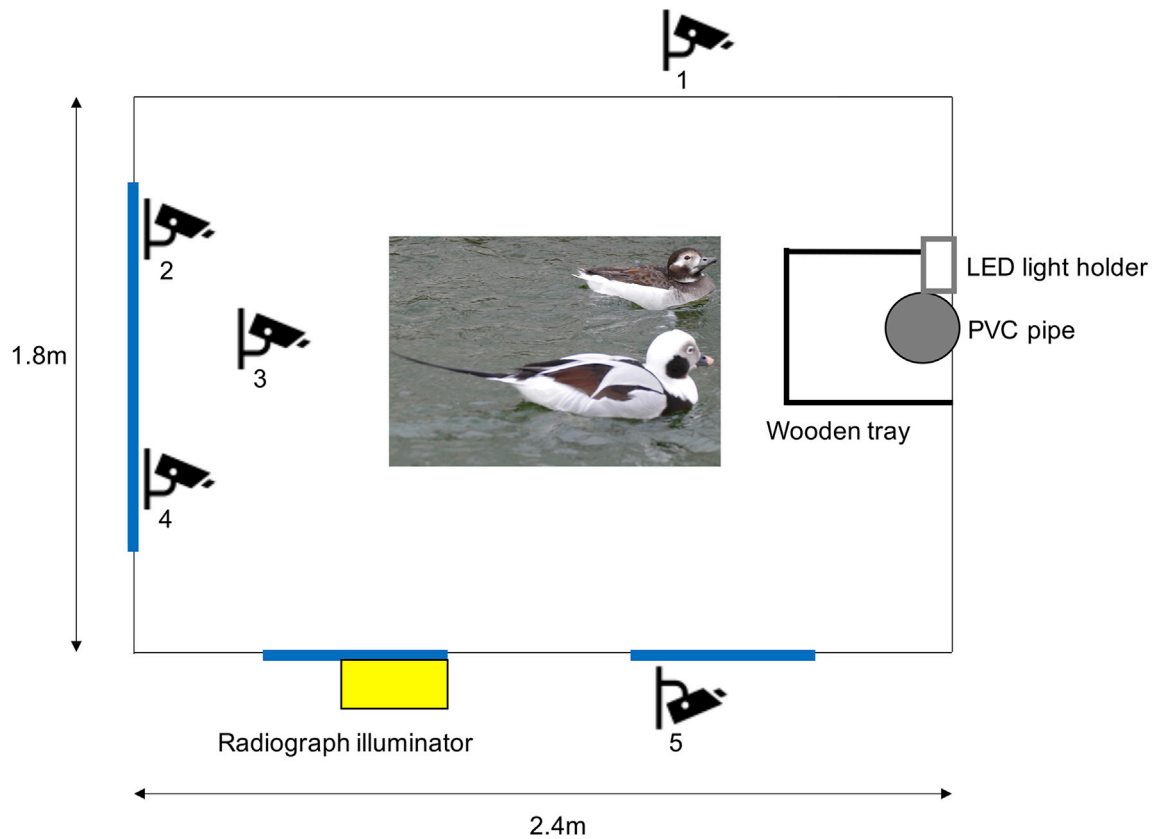
Fig. 1. Plan view of the experimental set up in the dive tank, with the Long-tailed Ducks swimming towards the food dispenser. There are 3 windows present in the dive tank (1 main window and 2 side windows), shown as lines on the tank walls, with the radiograph illuminator placed in one side window. The square wooden tray is on the bottom of the tank, with the PVC pipe and LED light holder positioned above the tray. Cameras 1 and 3 are located above the tank, cameras 2, 4 and 5 are placed on the windows of the dive tank, with camera 2 providing the video recording from the main window.
