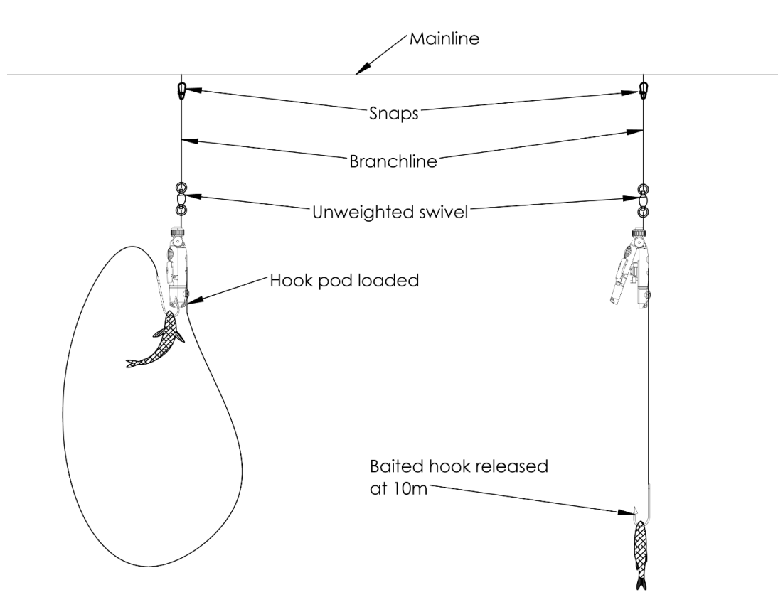
Figure 1: The Hookpod in situ prior to, and after, the pressure release mechanism opens the pod. Unweighted swivel is optional.
