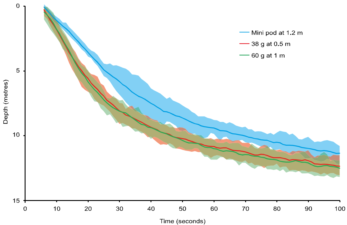
Figure 8: Sink rate results from vessel C. TDRs were placed 0.5 m from the hook on snoods with mini pods at 1.2 m from the hook (n=22), 38 g fixed swivels at 0.5 m (n=22), and 60 g
