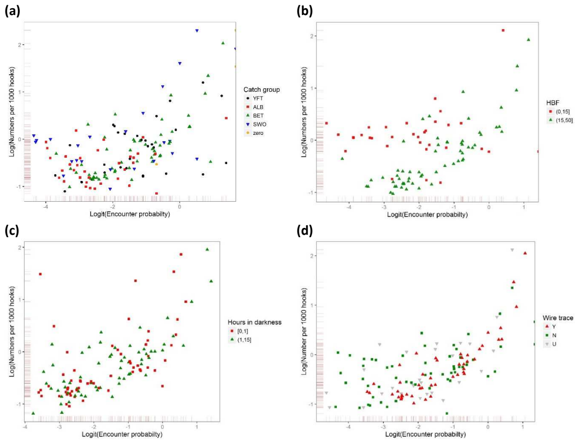
Figure E2: Relationships between encounter probabilities (in logit space) and BTH catch rates (in log space) in Core Area cells (2000–2014) as related to (a) catch group; (b) HBF (shallow sets ( HBF < 15 ) and deep sets ( HBF \geq 15 )); (c) fishing duration at night (hours in darkness); and (d) wire trace (“U” represents unknown).
