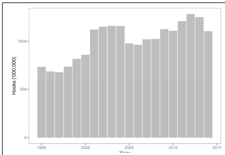
Figure 1: Total longline effort for the Pacific Ocean, 1995-2014 as downloaded from the SPC Catch Effort Query System (CES as of April 2016).
