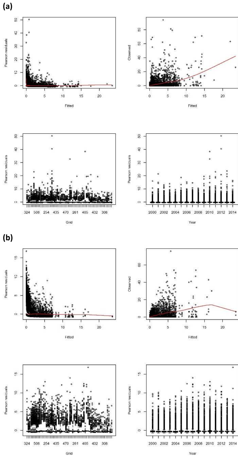
Figure E4: Residuals diagnostics for (a) the final ZINB (left) model fitted to Core Area observer data for the period 2000-2014; and (b) the same model fitted to simulated BTH catch data based on the predicted catch distribution derived from the final model. Pearson Residuals vs fitted values (top-left panel in both (a) and (b)); Observed catch vs fitted catch (top-right); Pearson Residuals by 5x5 degree cell (bottom-left); Pearson Residuals by year (bottom-right).
