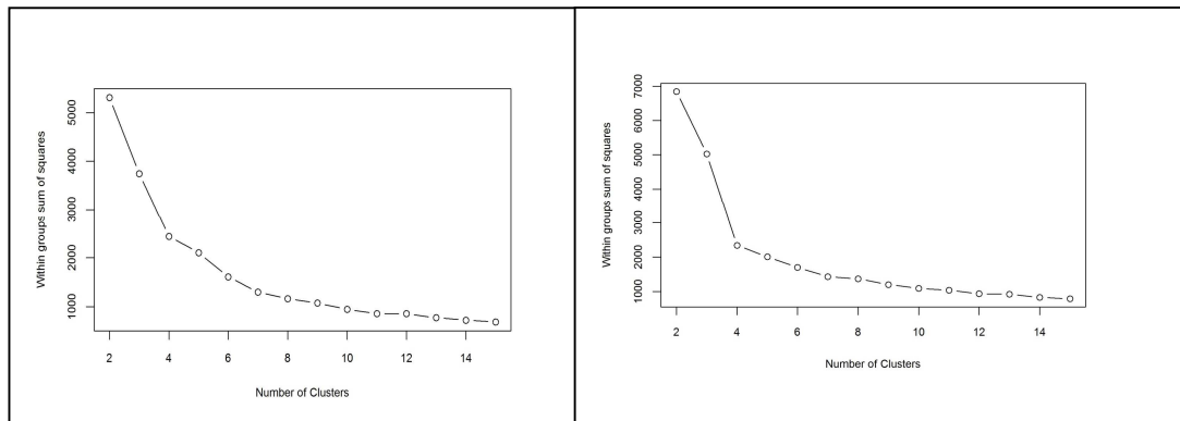
Figure 6: Diagnostics from kmeans cluster analysis showing the optimal number of targeting strategies based on the species composition of the longline catch for 1995-2004 (left) and 2005-2015 (right).
