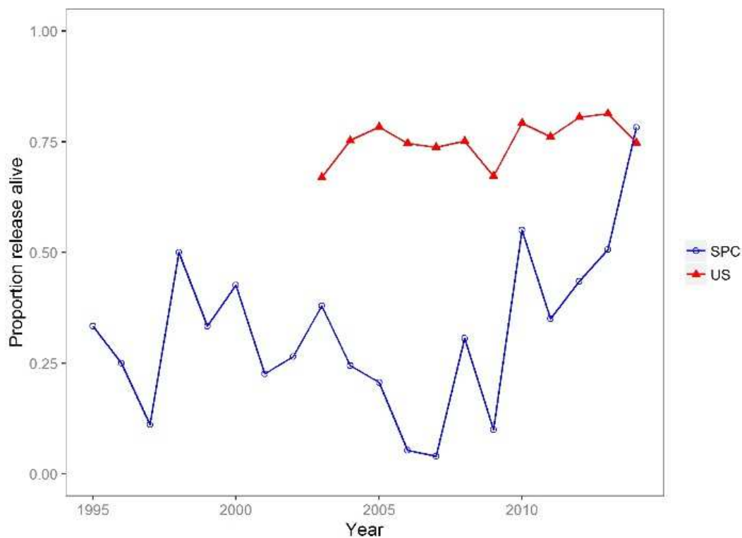
Figure 9: Annual proportion of BTH released alive for US observer data 2003–2014 and SPC observer data 1995–2014
