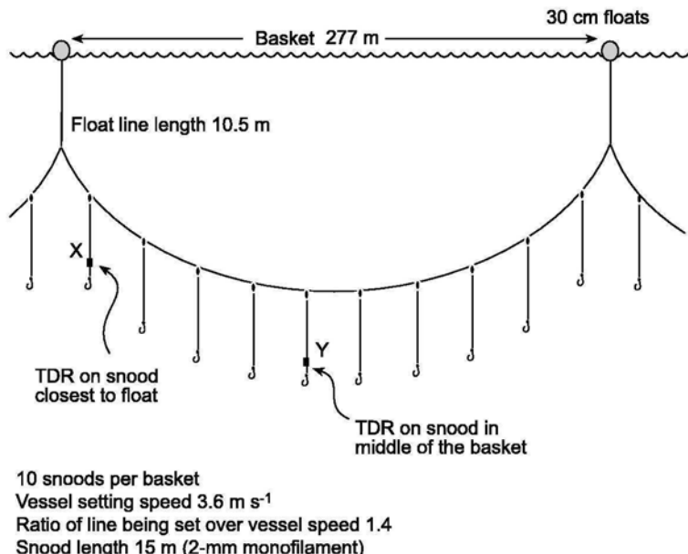
Fig. 1 F.V. Daniel Solander pelagic longline configuration. (TDR, time depth recorder.)
