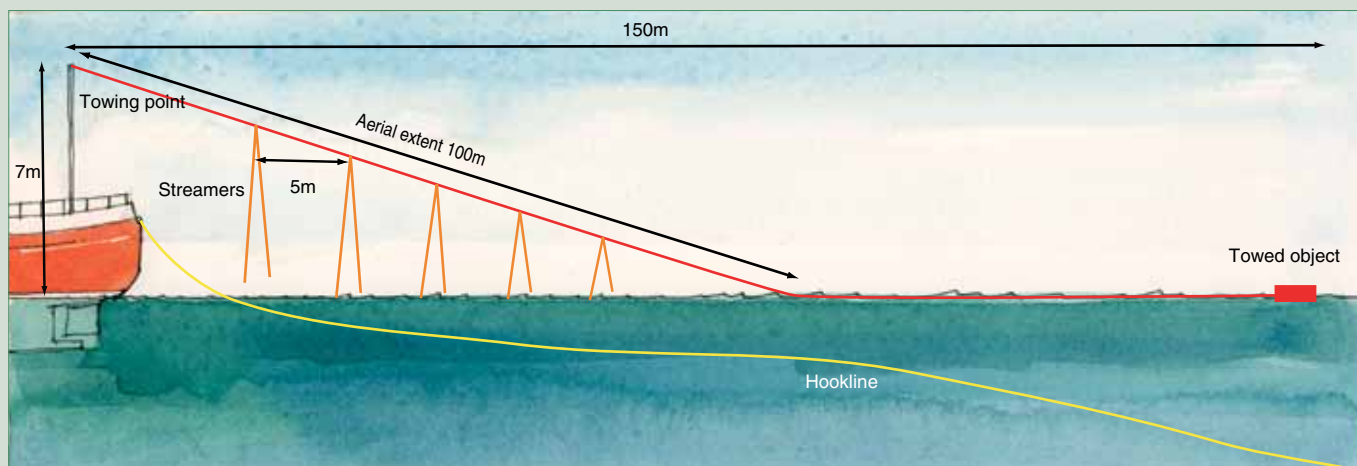
Figure 1. Typical structural and operational features of a streamer line.
