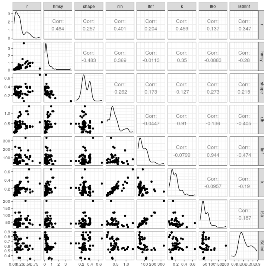
Figure 2. Relationships between r , H_{MSY} , and the shape of the Pella-Tomlinson production function from data-rich assessments, with data-poor estimates of r (r.lh) and life history parameters L_{\infty} , k and \frac{L_{50}}{L_{\infty}} .
