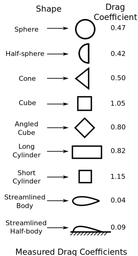
Figure 2. Measured drag coefficients for different shapes
