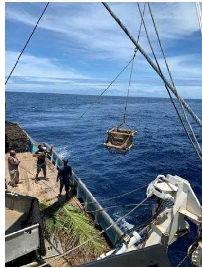
Figure 4. Trials in the western Pacific Ocean with the new FAD design
