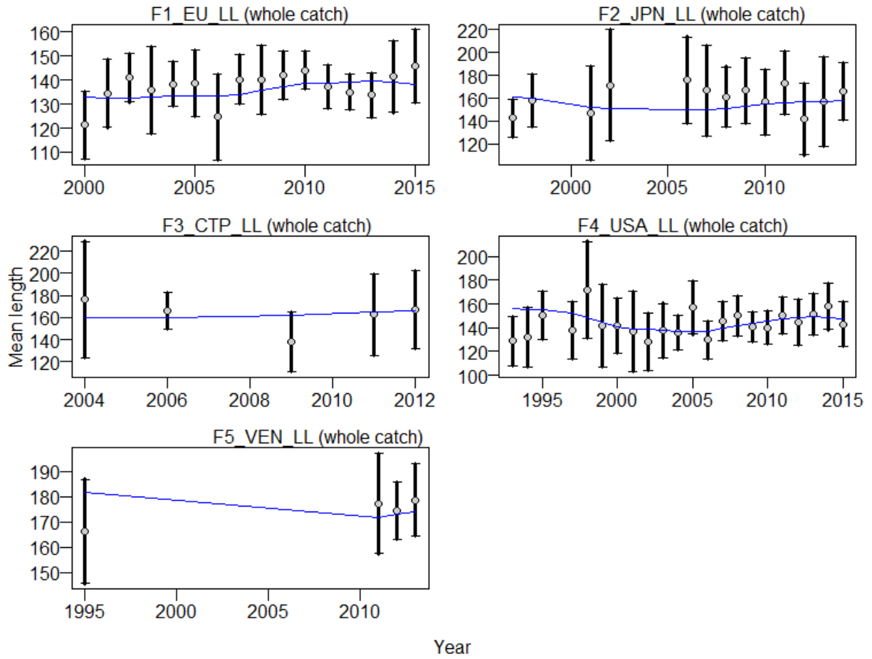
Figure 4. Mean length for Stock Synthesis model runs 1 (Panel A), 2 (Panel B), and 3 (Panel C). Fleets as defined in Table B.1 . Each subplot represents the input mean length by fleet (grey circle) and asymptotic 95% CI bars for years with input data along with the estimated mean length by fleet (blue line) from the integrated stock assessment model.
