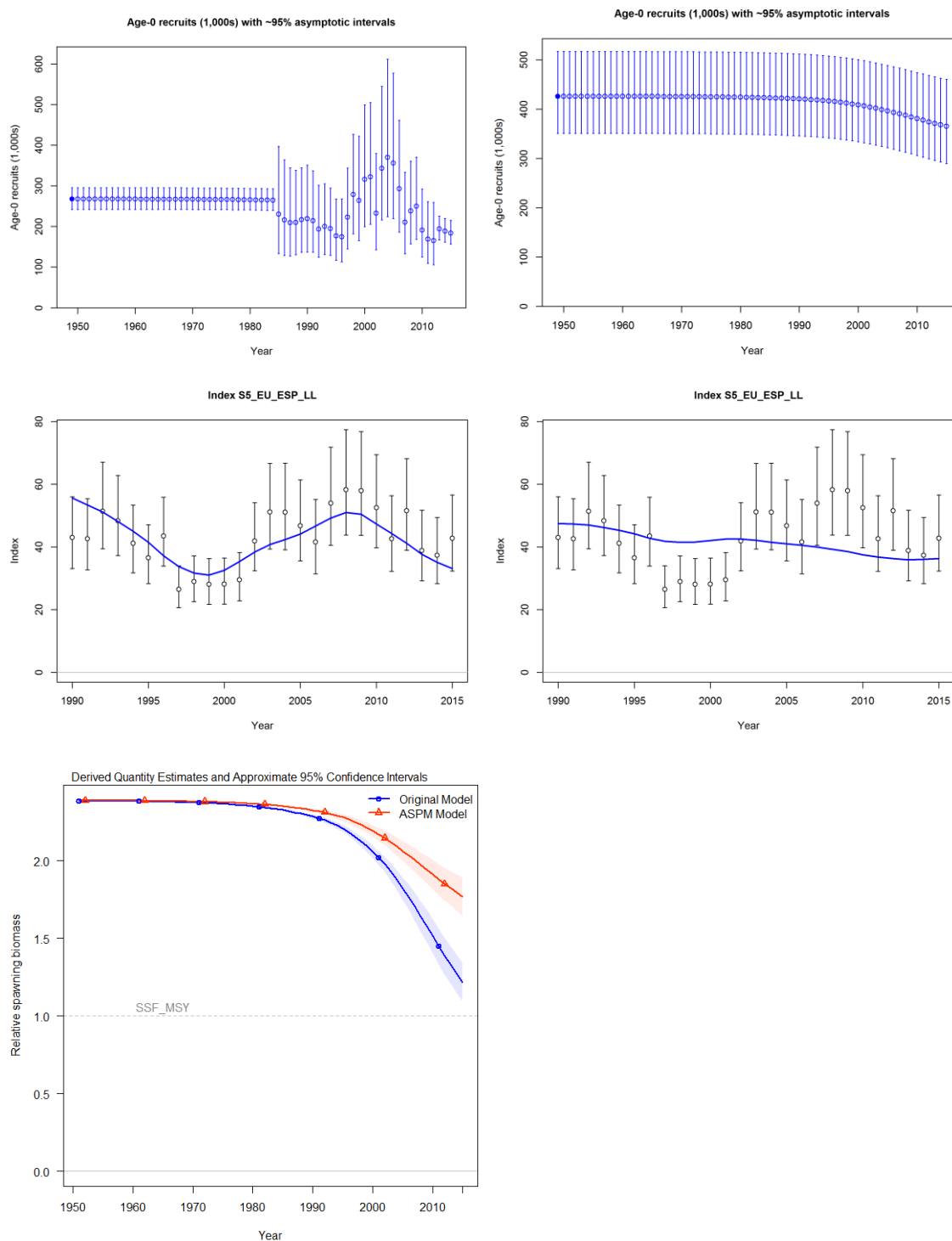
Figure 8. Age structured production model (ASPM) diagnostic for Stock Synthesis model runs 1 (Panel A), 2 (Panel B), and 3 (Panel C). Integrated stock assessment model age-0 recruits (upper left panel), ASPM model age-0 recruits (upper right panel), integrated stock assessment model fit to CPUE (EU ESP LL, middle left panel), ASPM model fit to CPUE (EU ESP LL, middle right panel), and relative spawning output (SSF/SSF_MSY, lower left panel) defined here as spawning stock fecundity (SSF), in units of pups produced per female, relative to SSF at MSY (SSF/SSF_MSY) from both the integrated stock assessment model and ASPM. Fleets as defined in Table B.1 .
