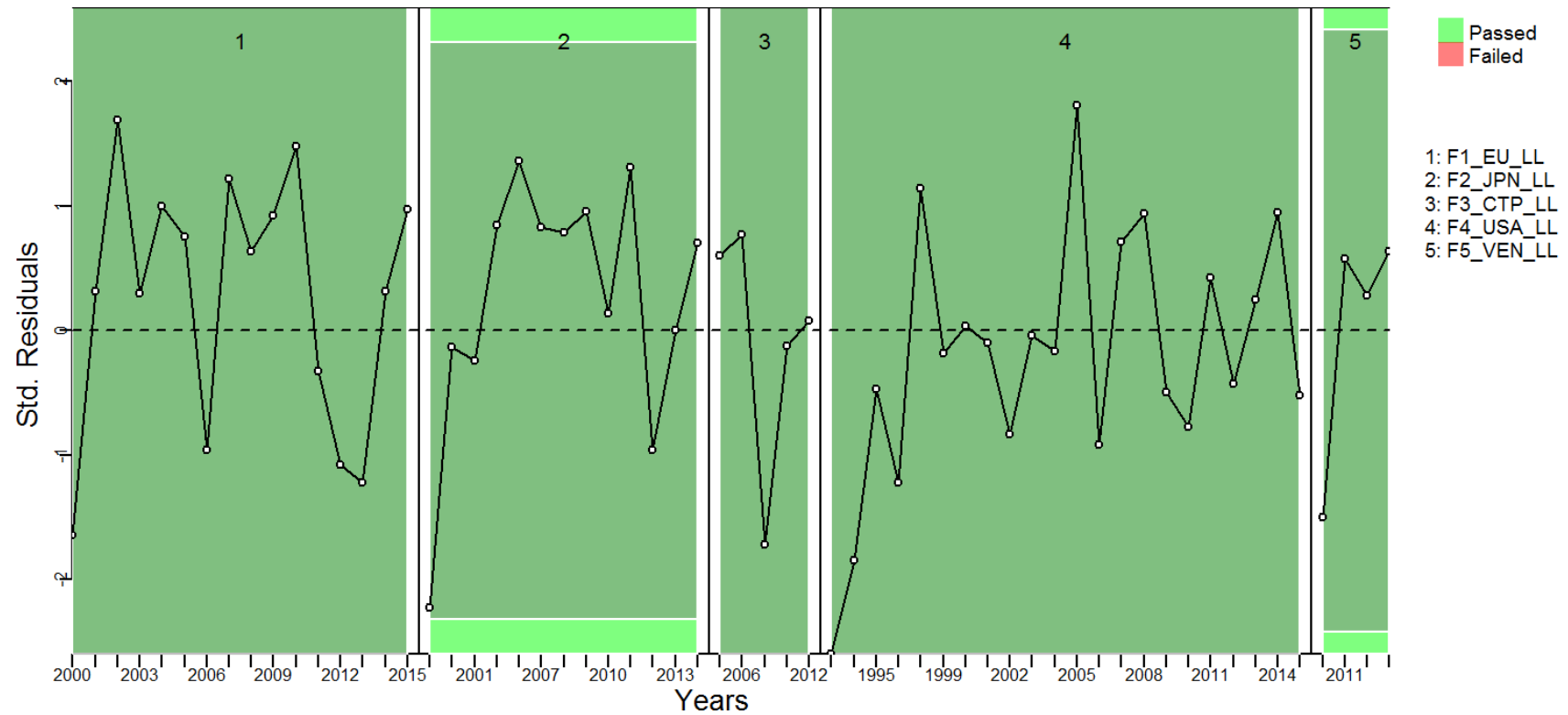
Figure 3. Runs tests on fits to mean length for Stock Synthesis model runs 1 (Panel A), 2 (Panel B), and 3 (Panel C). Fleets as defined in Table B.1 . Green background indicates no evidence ( p > 0.05 ) to reject the hypothesis of a randomly distributed time-series of residuals. Red background indicates evidence ( p < 0.05 ) to reject the hypothesis of randomly distributed residuals. Inner panels represent three standard errors from the mean. Red circles identify a residual greater than three standard errors from the mean.
