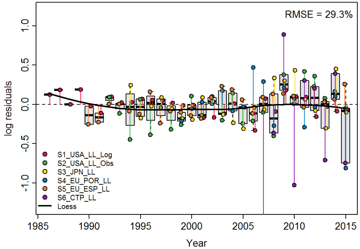
Figure 1. JABBA residual diagnostic plots for Stock Synthesis model runs 1 (Panel A), 2 (Panel B), and 3 (Panel C). Surveys as defined in Table B.1 . Boxplots as described in the methods section above.
