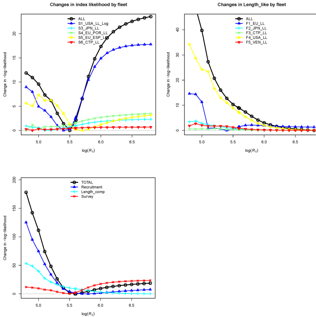
Figure 7. R_0 profiles for Stock Synthesis model runs 1 (Panel A), 2 (Panel B), and 3 (Panel C). Fleets as defined in Table B.1.
