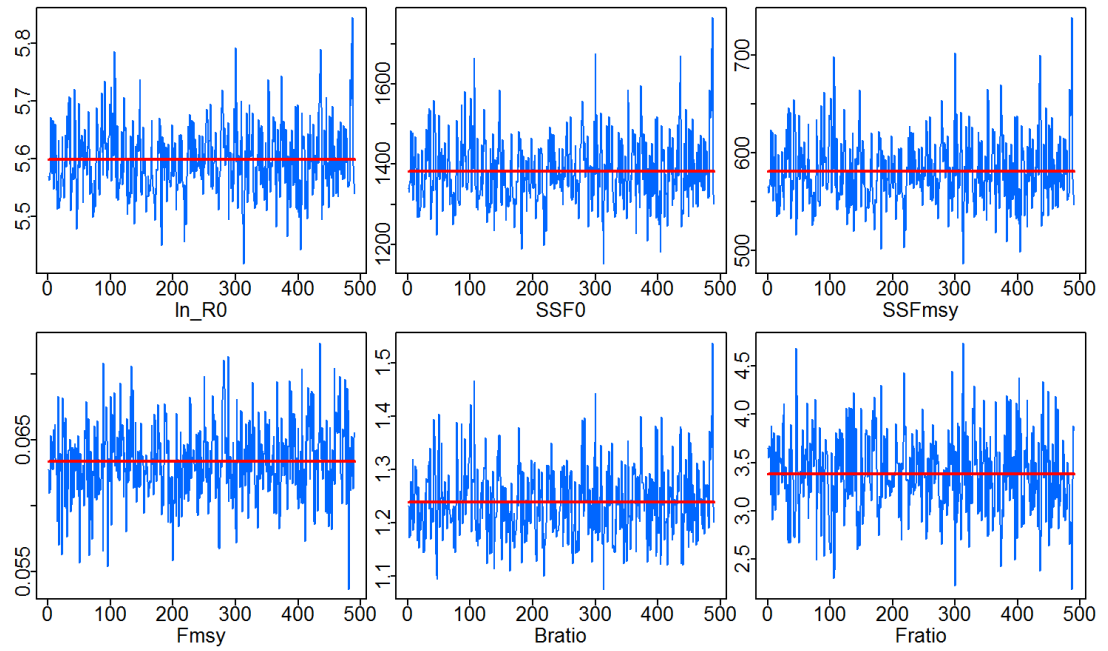
Figure 9. Short MCMC chains (as described in the methods) for Stock Synthesis model runs 1 (Panel A), 2 (Panel B), and 3 (Panel C) obtained for estimated parameters and derived quantities from Stock Synthesis output: 1) \log(R_0) ; 2) unfished spawning stock fecundity ( SSF_0 ); 3) spawning stock fecundity at MSY ( SSF_{MSY} ); 4) fishing mortality at MSY ( F_{MSY} ); 5) ending year spawning stock fecundity relative to its value at MSY ( SSF/SSF_{MSY} ); and 6) ending year fishing mortality relative to its value at MSY ( F/F_{MSY} ).
