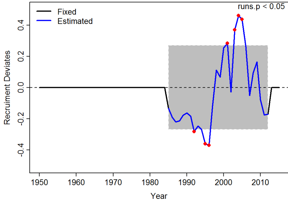
Figure 5. Runs tests on estimated recruitment deviates for Stock Synthesis model runs 1 (Panel A), 2 (Panel B), and 3 (Panel C) provide evidence ( \text{runs.p} < 0.05 ) to reject the hypothesis of randomly distributed estimated recruitment deviates. Inner panels represent three standard errors from the mean. Red circles identify a residual greater than three standard errors from the mean.
