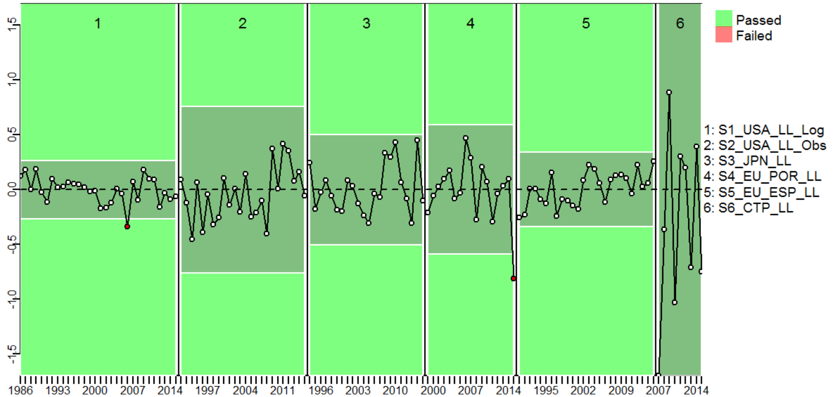
Figure 2. Runs tests on fits to CPUE for Stock Synthesis model runs 1 (Panel A), 2 (Panel B), and 3 (Panel C). Surveys as defined in Table B.1 . Green background indicates no evidence ( p > 0.05 ) to reject the hypothesis of a randomly distributed time-series of residuals. Red background indicates evidence ( p < 0.05 ) to reject the hypothesis of randomly distributed residuals. Inner panels represent three standard errors from the mean. Red circles identify a residual greater than three standard errors from the mean.
