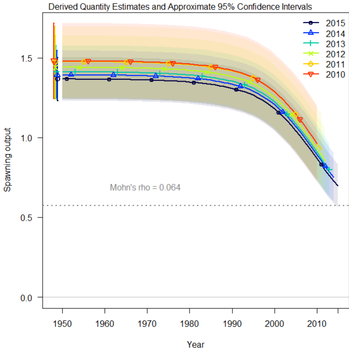
Figure 6. Retrospective analysis of spawning output for Stock Synthesis model runs 1 (Panel A), 2 (Panel B), and 3 (Panel C). Spawning output is spawning stock fecundity (SSF) in units of millions of pups produced. The stippled line is SSF at MSY. The Mohn's rho statistic is provided for the 5year peel.
