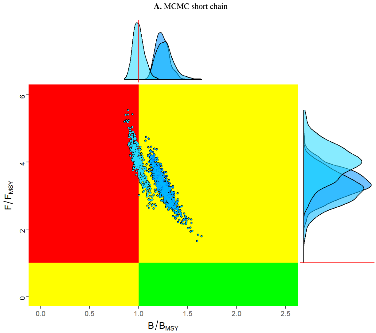
Figure 13. Kobe plot of MCMC short chain (Panel A) and long chain (Panel B) for Stock Synthesis model runs 1, 2, and 3. Runs 1 and 2 overlapped and differed from Run 3 (MCMC chain length as described in the methods).
