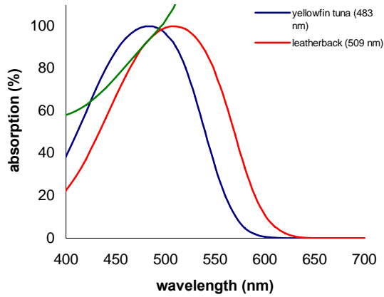
Figure 3: The spectral response curves of the rods of the two species with the greatest difference in \lambda_{max} . The green line shows the ratio of the quantum catch of the two as a function of wavelength. Even at 400 nm, the ratio is not dramatically different from 1 (100%), suggesting that selective invisibility based on special coloring is not likely to be very effective.
